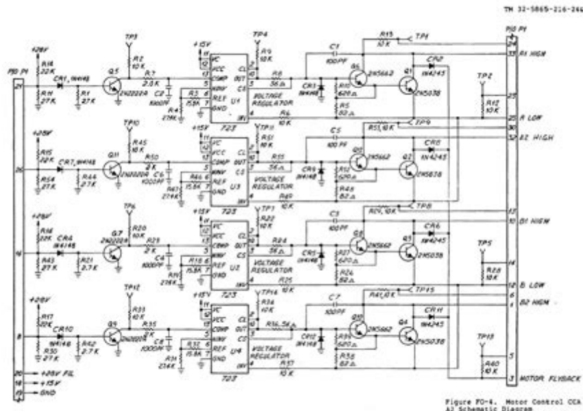
Figure PG-4. Motor Control CCA A2 Schematic Diagram
